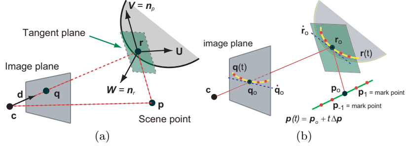
Fig. 2. Specular reflection geometry
