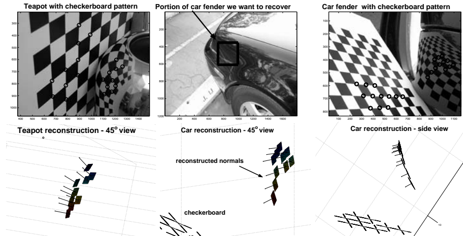
Fig. 5. Experimental results with real surfaces (teapot and car fender).
