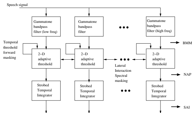
Figure 1: Auditory Image Model architecture. BMM = Basilar Membrane Motion, NAP = Neural Activity Pattern, SAI = Stabilized Auditory Image.
