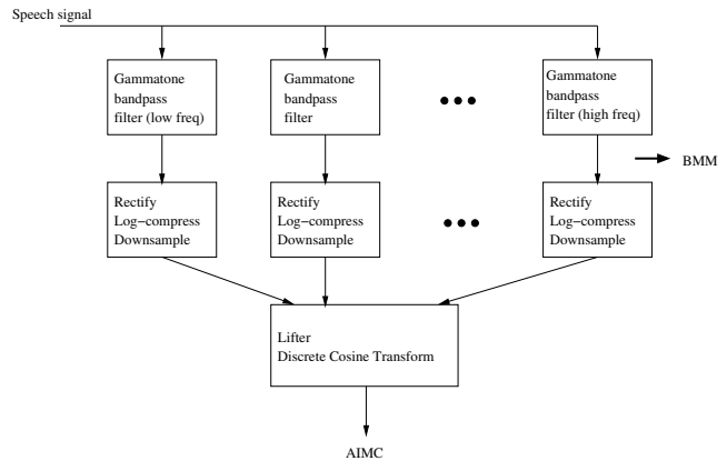
Figure 2: AIM Cepstrum (AIMC) computation flowchart.
